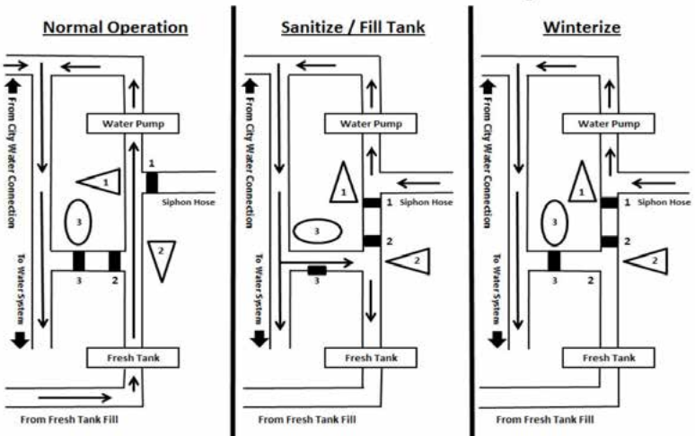
Fig. C - Flow Diagrams
