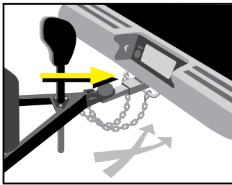
3. Connect passenger side chain to driver side mounting point on tow vehicle hitch. Chains should cross but not touch the ground.
