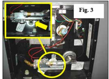
Water heater drain plug location
