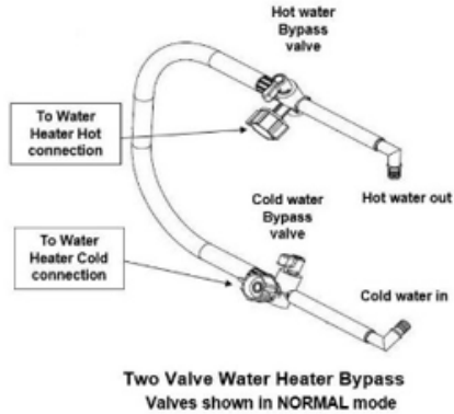
Fig. B - Water Heater Bypass (2 valves)
