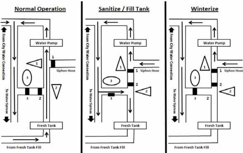
Fig. C - Flow Diagrams
